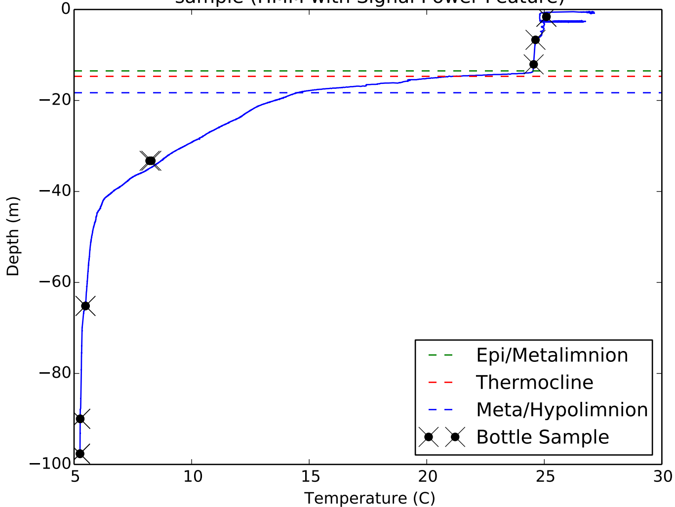
sample (HMM with Signal Power Feature)
